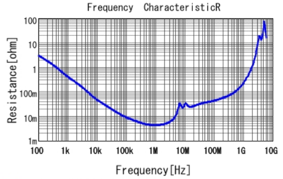
■ GRM43ER72A225KA01 R DCOV, 25degC
