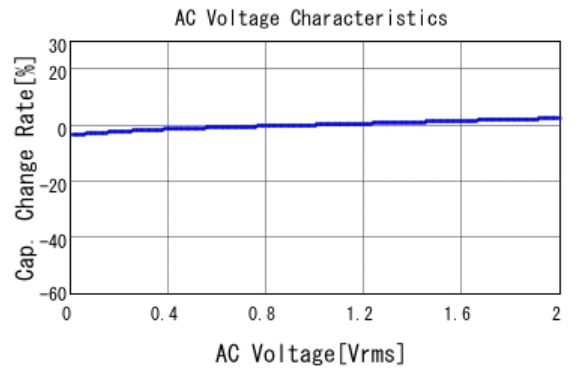
■ GRM43ER72A225KA01 C-AC Voltage capchange, DCOV, 25.0d
