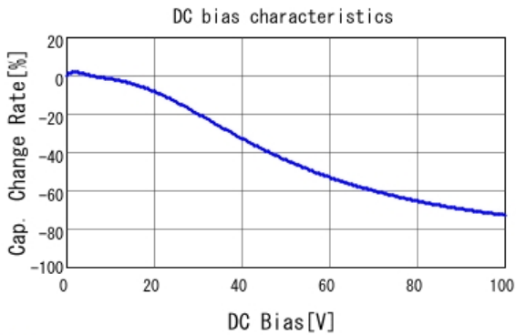
■ GRM43ER72A225KA01 C-DC bias capchange, 25.0degC, AC1.
