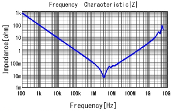
■ GRM43ER72A225KA01 |Z| DCOV, 25degC
