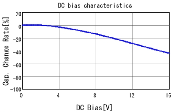
■ GRM43ER61C226ME01 C-DC bias capchange, 25.0degC, AC0.
