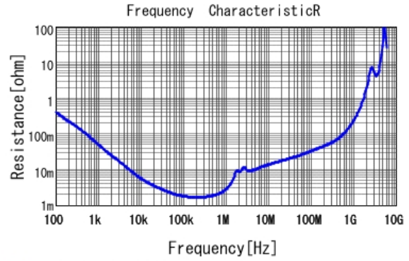
■ GRM43ER61C226ME01 R DCOV, 25degC
