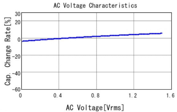
■ GRM43ER61C226ME01 C-AC Voltage capchange, DCOV, 25.0d
