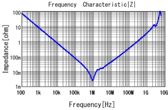
■ GRM43ER61C226ME01 |Z| DCOV, 25degC
