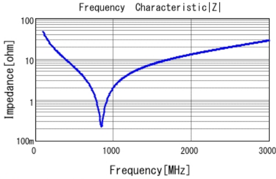
■ GRM42A7U3F330JW31 |Z| DC0V, 25degC
