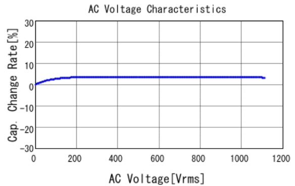
■ GRM42A7U3F330JW31 C-AC Voltage capchange, DC0V, 25.0d
