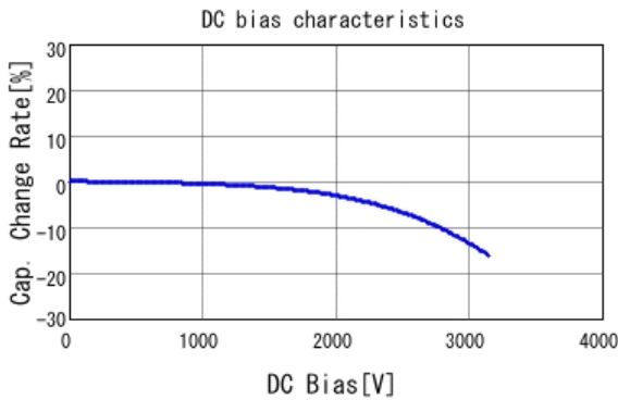
■ GRM42A7U3F330JW31 C-DC bias capchange, 25.0degC, AC1V
