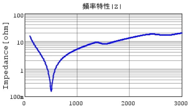
GRM42A7U3F101JW31 |Z| DCOV, 25degC
