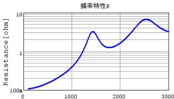
GRM42A7U3F101JW31 R DCOV, 25degC
