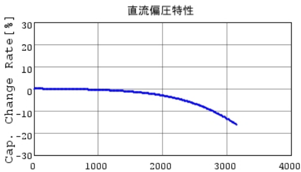
GRM42A7U3F101JW31 C-DC bias capchange, 25.0c
