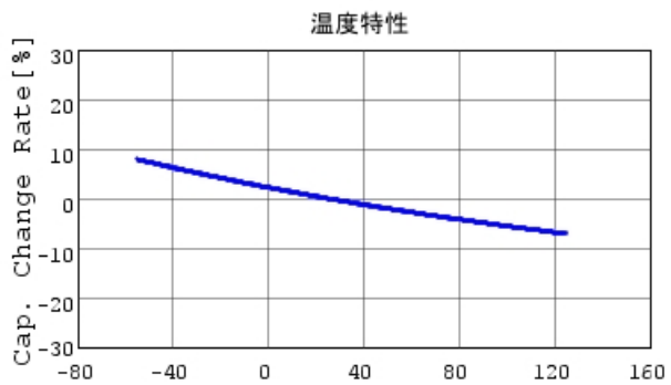
GRM42A7U3F101JW31 C-Temp. capchange, DCOV, #
