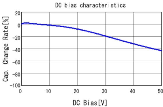
■ GRM32RB11H105KA01 C-DC bias capchange, 20.0degC, AC1.
