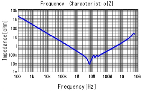
■ GRM32RB11H105KA01 |Z| DCOV, 20degC
