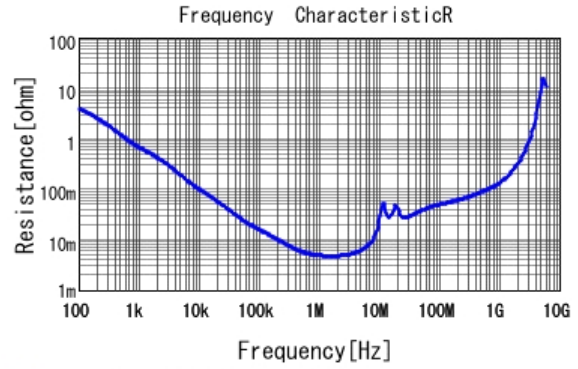
■ GRM32RB11H105KA01 R DCOV, 20degC
