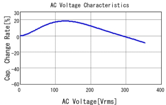
■ GRM32QR73A682KW01 C-AC Voltage capchange, DCOV, 25.0d
