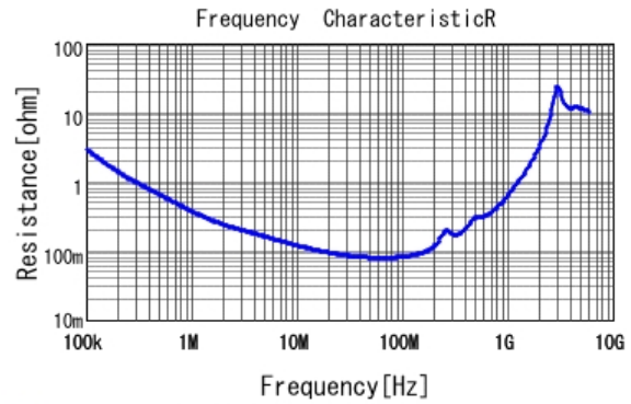
■ GRM32QR73A682KW01 R DCOV, 25degC
