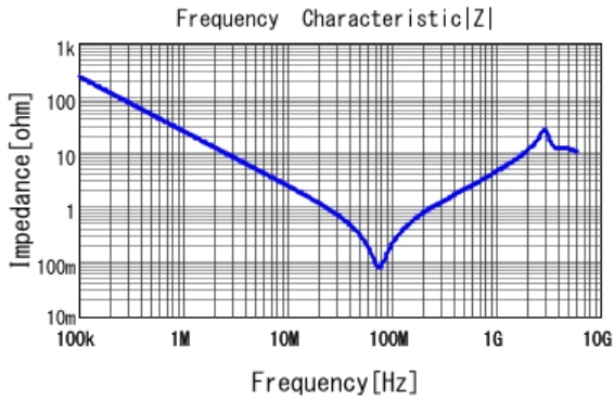
■ GRM32QR73A682KW01 |Z| DCOV, 25degC
