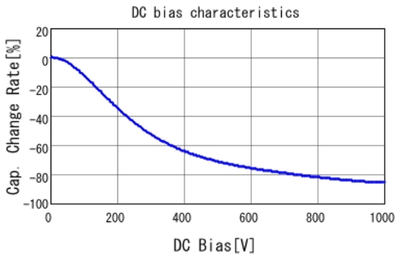
■ GRM32QR73A682KW01 C-DC bias capchange, 25.0degC, AC1V
