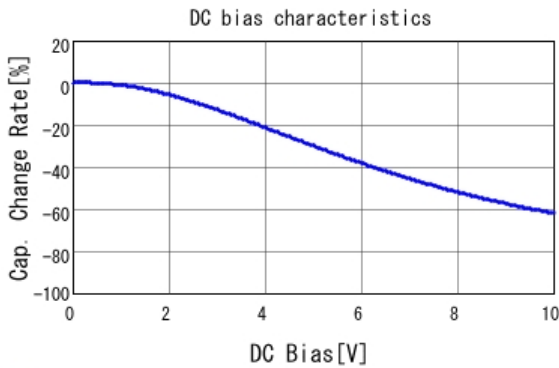
■ GRM32NR61A226KE19 C-DC bias capchange, 25.0degC, AC0.
