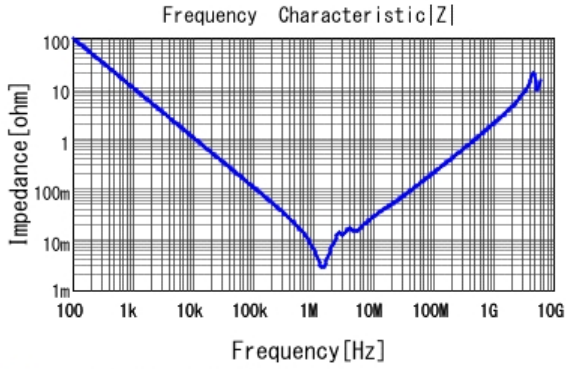
■ GRM32NR61A226KE19 |Z| DCOV, 25degC
