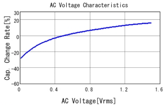
■ GRM32NR61A226KE19 C-AC Voltage capchange, DCOV, 25.0d
