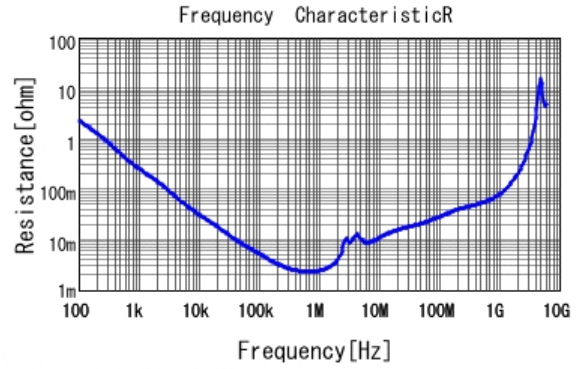
■ GRM32NR61A226KE19 R DCOV, 25degC
