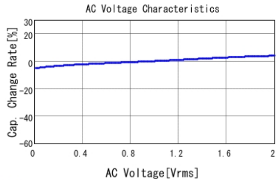
■ GRM32MR71C225KA01 C-AC Voltage capchange, DCOV, 25.0d
