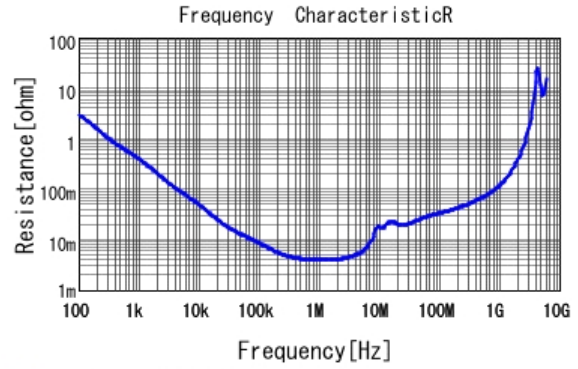
■ GRM32MR71C225KA01 R DCOV, 25degC
