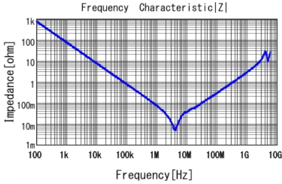
■ GRM32MR71C225KA01 |Z| DCOV, 25degC
