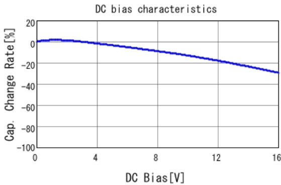
■ GRM32MR71C225KA01 C-DC bias capchange, 25.0degC, AC1.
