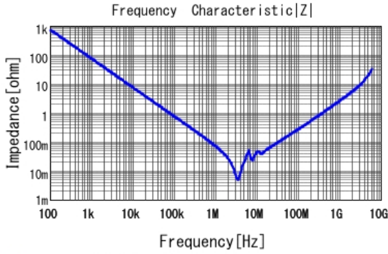
■ GRM32ER72A225MA35 |Z| DCOV, 25degC
