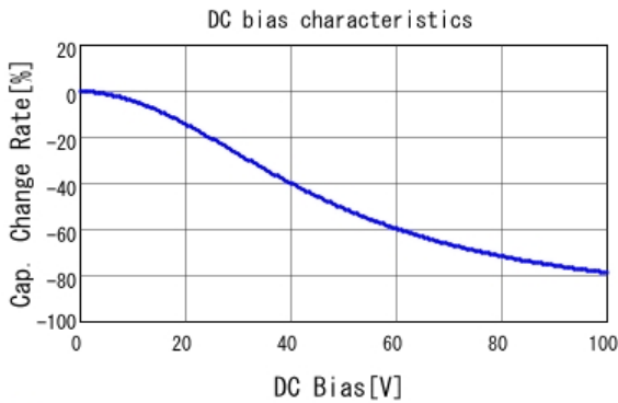
■ GRM32ER72A225MA35 C-DC bias capchange, 25.0degC, AC1.
