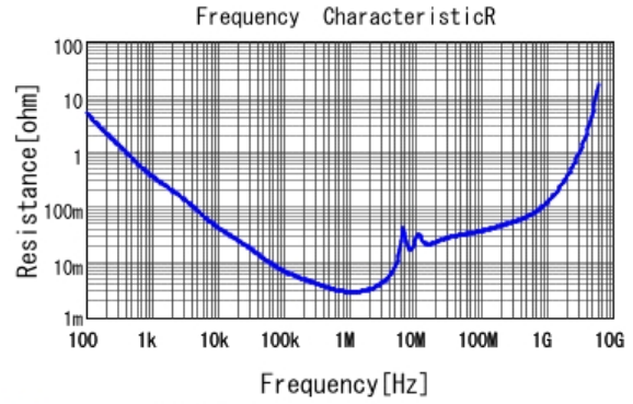
■ GRM32ER72A225MA35 R DCOV, 25degC
