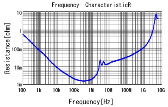
■ GRM32ER71J106KA12 R DCOV, 25degC
