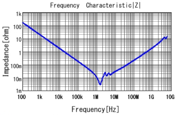
■ GRM32ER71J106KA12 |Z| DCOV, 25degC
