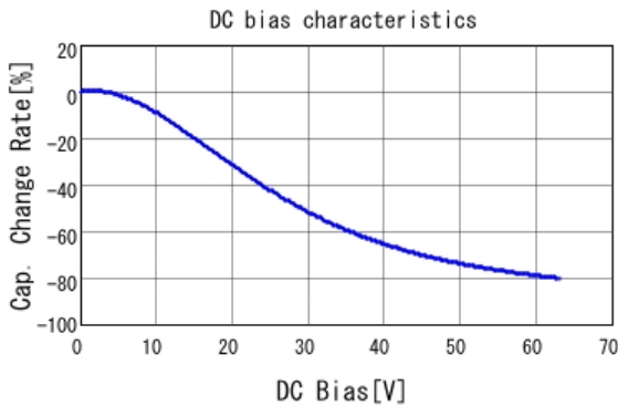
■ GRM32ER71J106KA12 C-DC bias capchange, 25.0degC, AC1V
