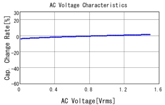
■ GRM32ER71J106KA12 C-AC Voltage capchange, DCOV, 25.0d
