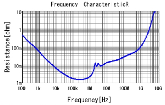
■ GRM32ER71A226ME20 R DCOV, 25degC
