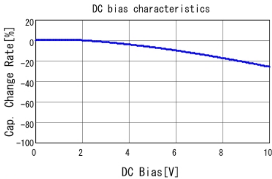
■ GRM32ER71A226ME20 C-DC bias capchange, 25.0degC, AC0.
