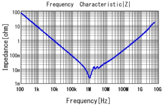
■ GRM32ER71A226ME20 |Z| DCOV, 25degC
