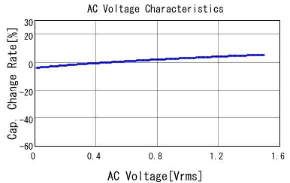
■ GRM32ER71A226ME20 C-AC Voltage capchange, DCOV, 25.0d
