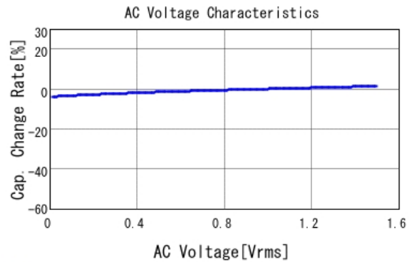
■ GRM32ER6YA106MA12 C-AC Voltage capchange, DCOV, 25.0d
