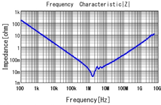
■ GRM32ER6YA106MA12 |Z| DCOV, 25degC
