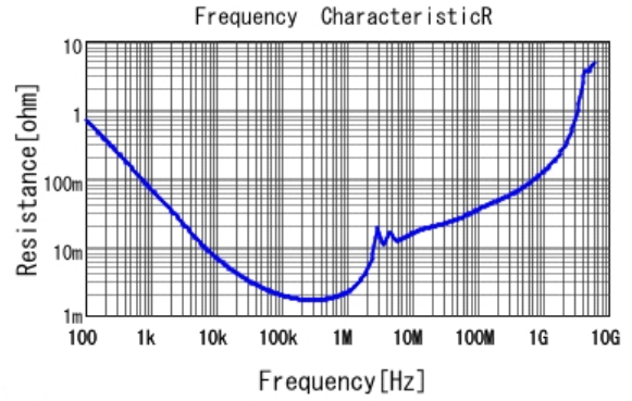
■ GRM32ER6YA106MA12 R DCOV, 25degC
