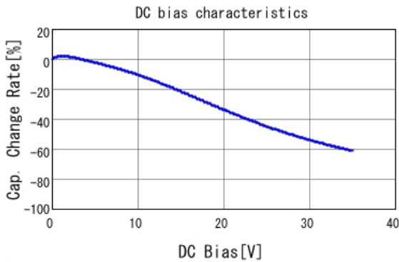
■ GRM32ER6YA106MA12 C-DC bias capchange, 25.0degC, AC1.
