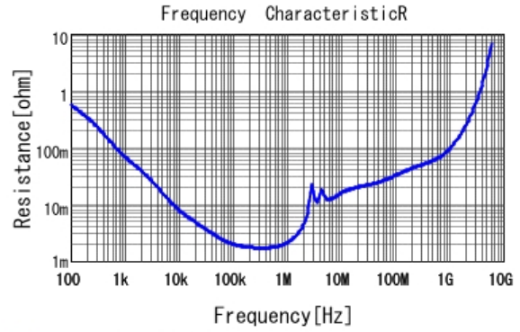
■ GRM32ER6YA106KA12 R DCOV, 25degC
