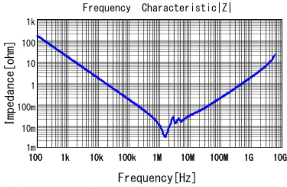
■ GRM32ER6YA106KA12 |Z| DCOV, 25degC
