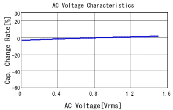
■ GRM32ER6YA106KA12 C-AC Voltage capchange, DCOV, 25.0d
