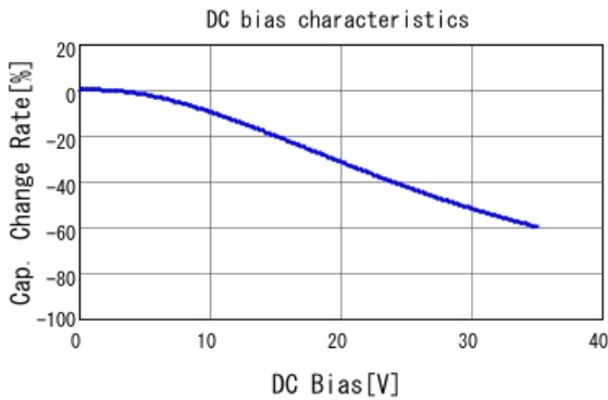
■ GRM32ER6YA106KA12 C-DC bias capchange, 25.0degC, AC1.
