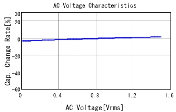
■ GRM32ER61H106MA12 C-AC Voltage capchange, DCOV, 25.0d
