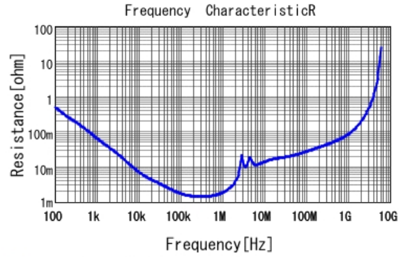
■ GRM32ER61H106MA12 R DCOV, 25degC
