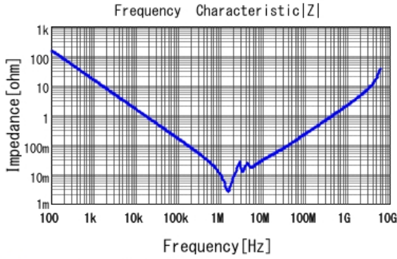
■ GRM32ER61H106MA12 |Z| DCOV, 25degC
