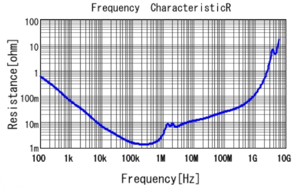
■ GRM32ER60J476ME64 R DCOV, 25degC
