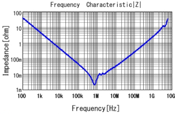
■ GRM32ER60J476ME64 |Z| DCOV, 25degC
