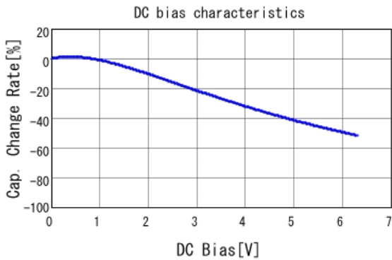
■ GRM32ER60J476ME64 C-DC bias capchange, 25.0degC, AC0.
