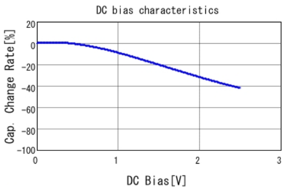
■ GRM32ER60E337ME05 C-DC bias capchange, 25.0degC, AC0.
