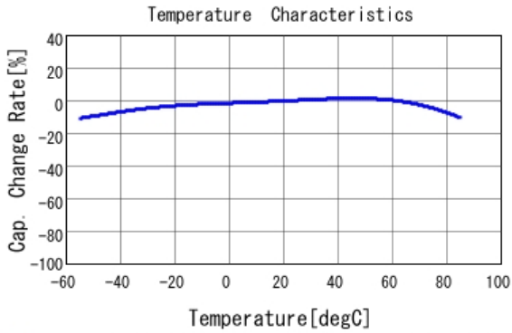
■ GRM32ER60E337ME05 C-Temp. capchange, DC0.0V, AC0.15Vr
