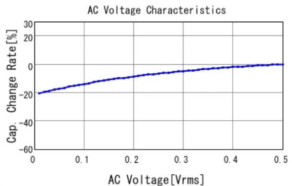
■ GRM32ER60E337ME05 C-AC Voltage capchange, DCOV, 25.0d
