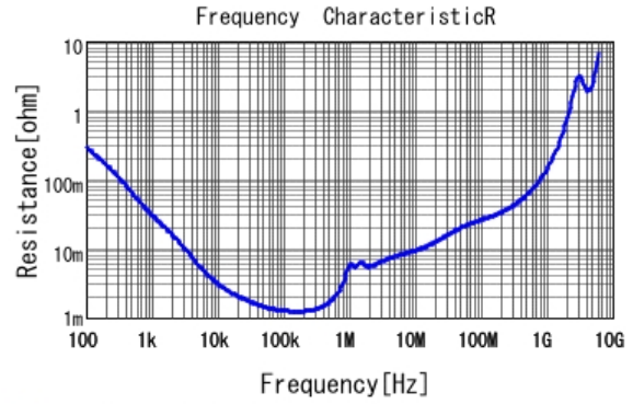
■ GRM32EE70J107ME15 R DCOV, 25degC
