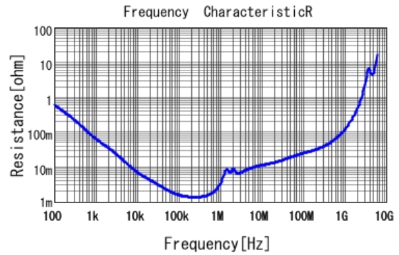
■ GRM32ED71A476KE15 R DCOV, 25degC
