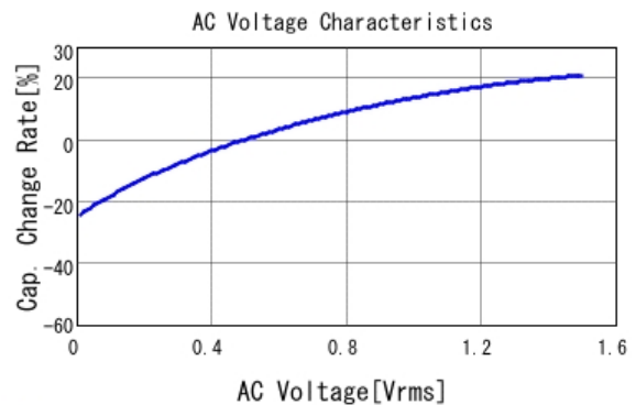
■ GRM32ED71A476KE15 C-AC Voltage capchange, DCOV, 25.0d
