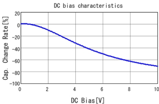
■ GRM32ED71A476KE15 C-DC bias capchange, 25.0degC, AC0.
