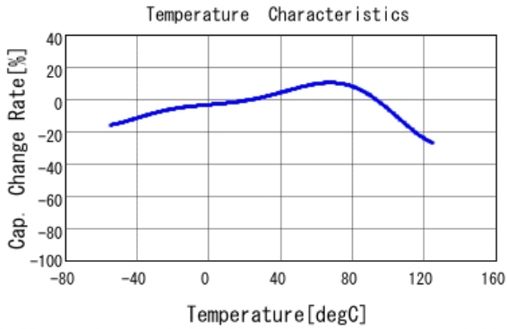
■ GRM32ED71A476KE15 C-Temp. capchange, DC0.0V, AC0.3Vrm
