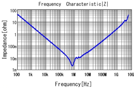
■ GRM32ED71A476KE15 |Z| DCOV, 25degC
