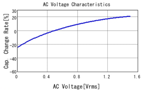
■ GRM32ED70J476KE20 C-AC Voltage capchange, DCOV, 25.0d
