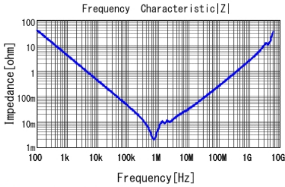
■ GRM32ED70J476KE20 |Z| DCOV, 25degC
