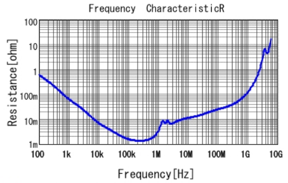
■ GRM32ED70J476KE20 R DCOV, 25degC
