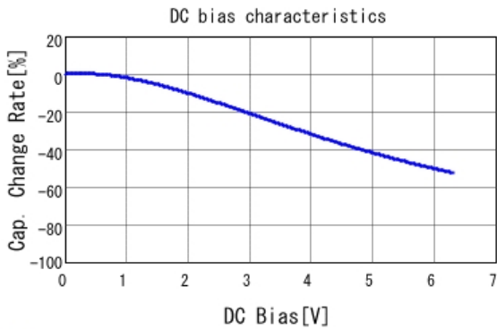
■ GRM32ED70J476KE20 C-DC bias capchange, 25.0degC, AC0.
