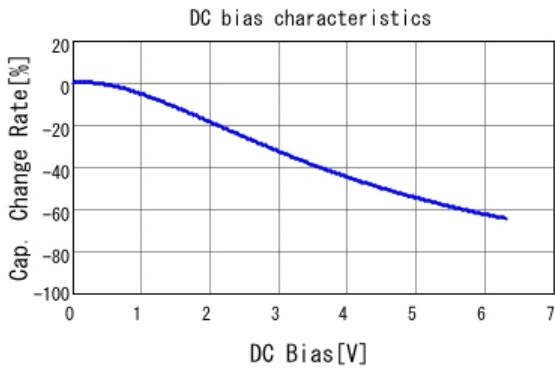
■ GRM32EC80J107ME20 C-DC bias capchange, 25.0degC, AC0.
