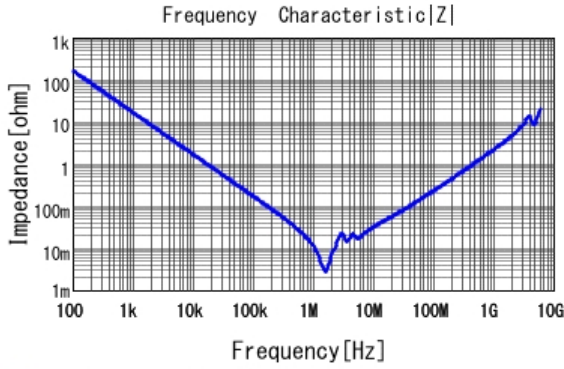
■ GRM32EC72A106KE05 |Z| DCOV, 25degC
