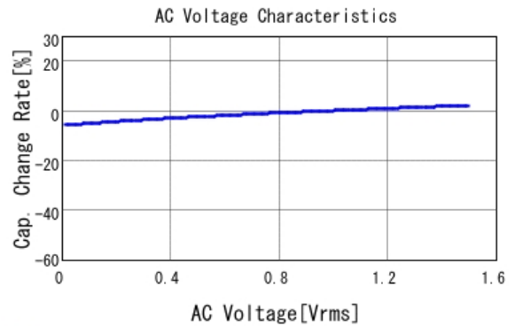
■ GRM32EC72A106KE05 C-AC Voltage capchange, DCOV, 25.0d
