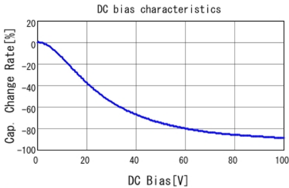
■ GRM32EC72A106KE05 C-DC bias capchange, 25.0degC, AC1V
