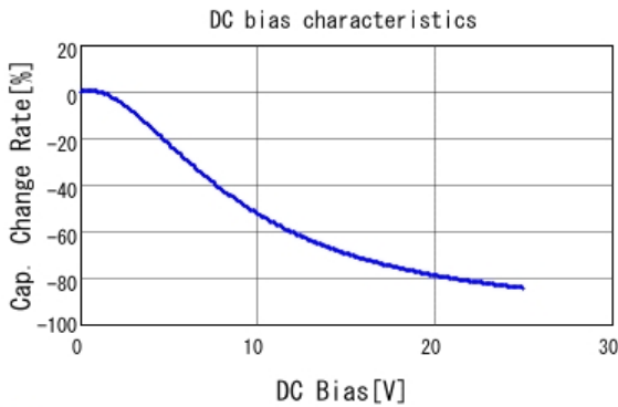
■ GRM32EB31E226ME15 C-DC bias capchange, 20.0degC, AC0.
