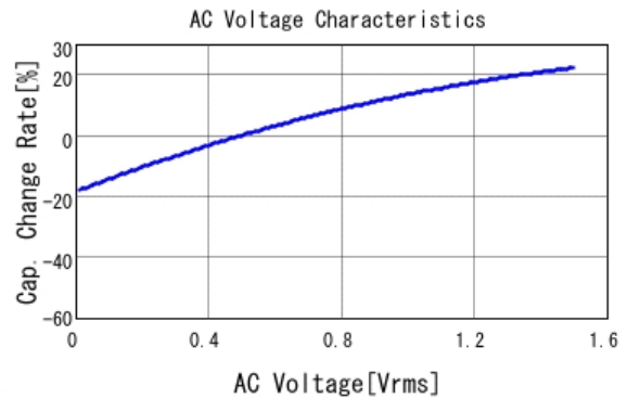
■ GRM32EB31E226ME15 C-AC Voltage capchange, DCOV, 20.0d
