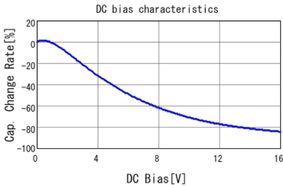
■ GRM32EB31C476KE15 C-DC bias capchange, 20.0degC, AC0.
