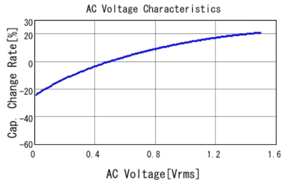
■ GRM32EB31C476KE15 C-AC Voltage capchange, DCOV, 20.0d
