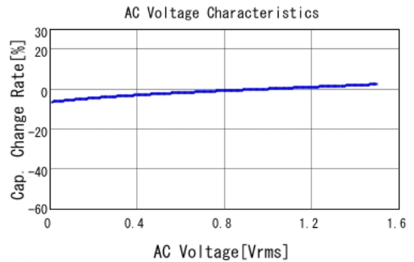
■ GRM32DR61E106KA12 C-AC Voltage capchange, DCOV, 25.0d
