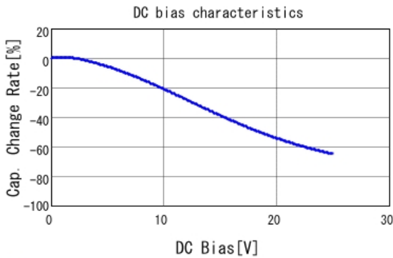
■ GRM32DR61E106KA12 C-DC bias capchange, 25.0degC, AC1.
