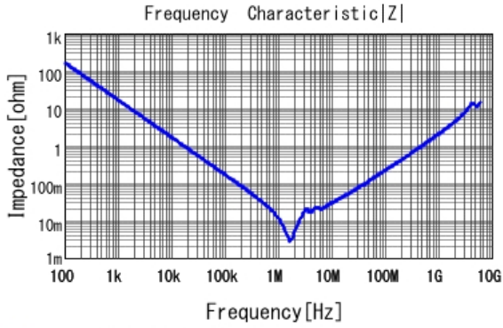
■ GRM32DR61E106KA12 |Z| DCOV, 25degC
