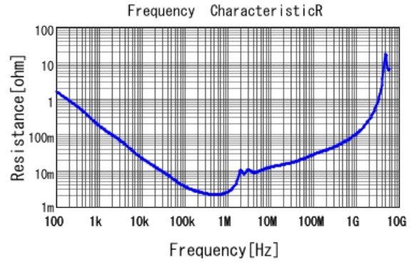
■ GRM32DR60J336ME19 R DCOV, 25degC
