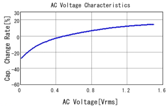
■ GRM32DR60J336ME19 C-AC Voltage capchange, DCOV, 25.0d
