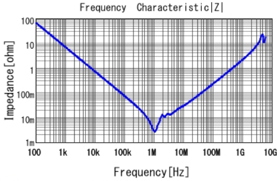
■ GRM32DR60J336ME19 |Z| DCOV, 25degC
