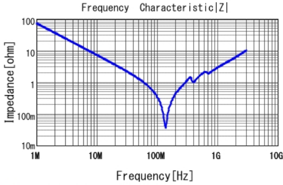
■ GRM32A7U2J222JW31 |Z| DCOV, 25degC
