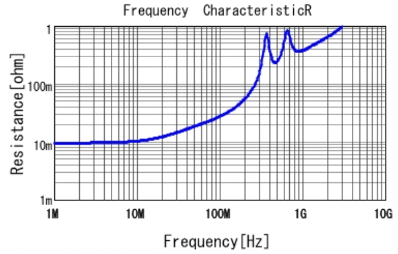
■ GRM32A7U2J222JW31 R DCOV, 25degC
