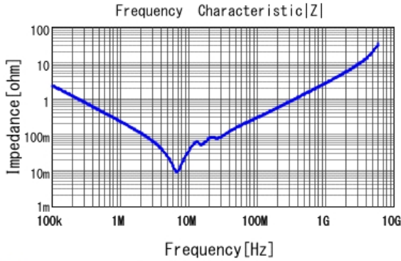
■ GRM31MR72A684KA35 |Z| DCOV, 25degC
