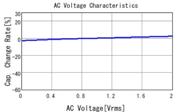
■ GRM31MR72A684KA35 C-AC Voltage capchange, DCOV, 25.0d
