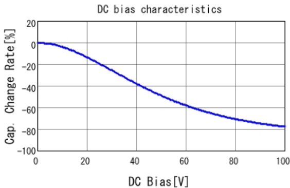
■ GRM31MR72A684KA35 C-DC bias capchange, 25.0degC, AC1.
