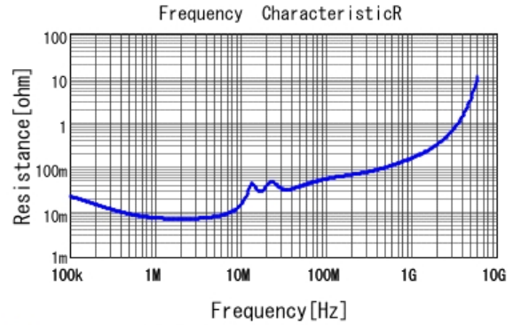
■ GRM31MR72A684KA35 R DCOV, 25degC
