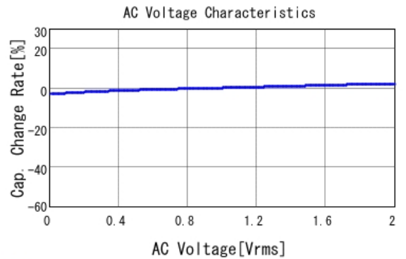
■ GRM31MR72A154KA01 C-AC Voltage capchange, DCOV, 25.0d
