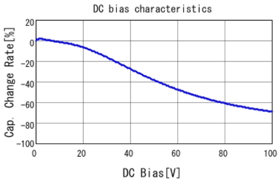
■ GRM31MR72A154KA01 C-DC bias capchange, 25.0degC, AC1.
