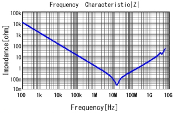
■ GRM31MR72A154KA01 |Z| DCOV, 25degC
