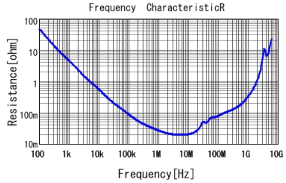
■ GRM31MR72A154KA01 R DCOV, 25degC
