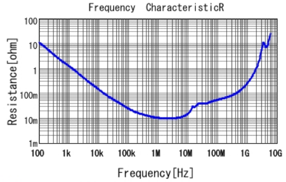
■ GRM31MR71H684KA88 R DCOV, 25degC
