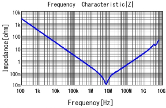
■ GRM31MR71H684KA88 |Z| DCOV, 25degC
