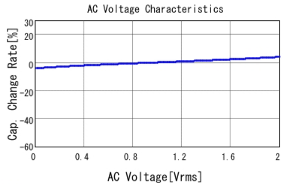
■ GRM31MR71H684KA88 C-AC Voltage capchange, DCOV, 25.0d
