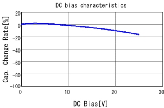
■ GRM31MR71E474KA01 C-DC bias capchange, 25.0degC, AC1.
