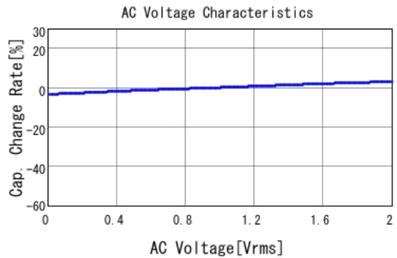
■ GRM31MR71E474KA01 C-AC Voltage capchange, DCOV, 25.0d
