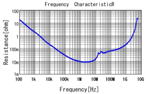
■ GRM31MR71E474KA01 R DCOV, 25degC
