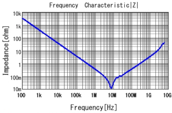
■ GRM31MR71E474KA01 |Z| DCOV, 25degC
