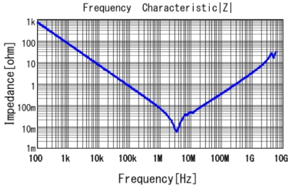
■ GRM31MR71C225KA35 |Z| DCOV, 25degC
