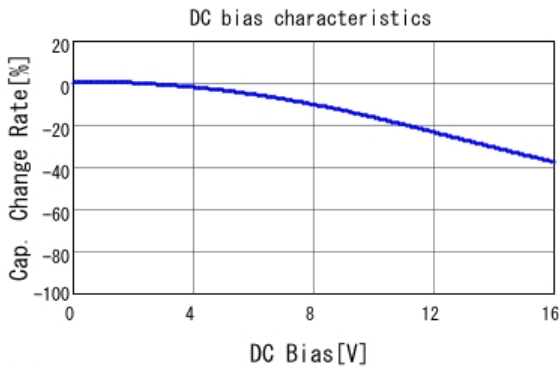
■ GRM31MR71C225KA35 C-DC bias capchange, 25.0degC, AC1.
