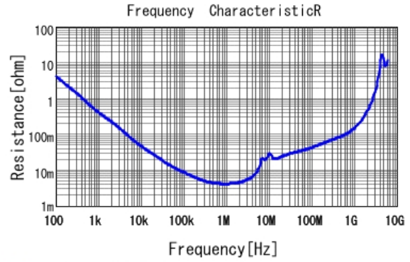
■ GRM31MR71C225KA35 R DCOV, 25degC
