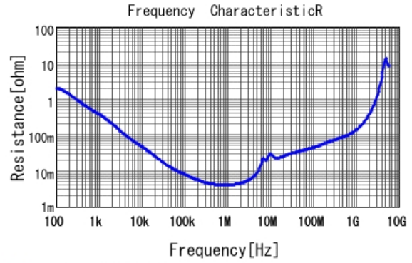
■ GRM31MR71A225KA01 R DCOV, 25degC
