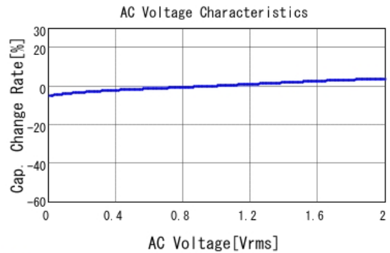
■ GRM31MR71A225KA01 C-AC Voltage capchange, DCOV, 25.0d
