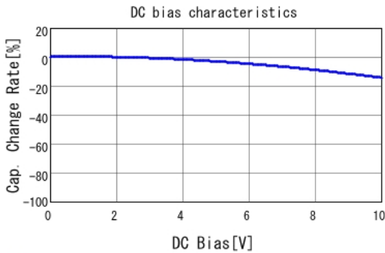
■ GRM31MR71A225KA01 C-DC bias capchange, 25.0degC, AC1.
