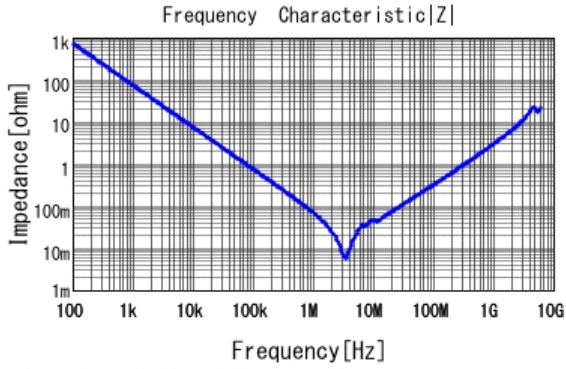
■ GRM31MR71A225KA01 |Z| DCOV, 25degC
