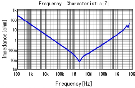
■ GRM31MR61E106MA12 |Z| DCOV, 25degC
