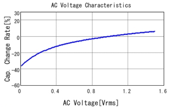
■ GRM31MR61E106MA12 C-AC Voltage capchange, DCOV, 25.0d
