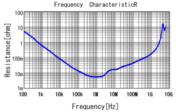
■ GRM31MR61E106MA12 R DCOV, 25degC
