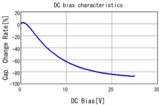
■ GRM31MR61E106MA12 C-DC bias capchange, 25.0degC, AC1.
