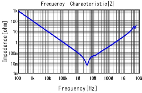
■ GRM31MR61C225KA35 |Z| DCOV, 25degC
