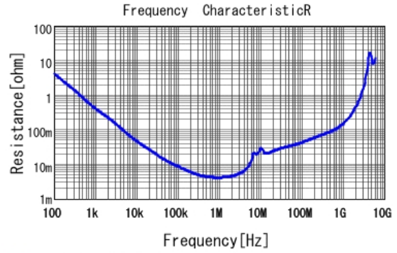
■ GRM31MR61C225KA35 R DCOV, 25degC
