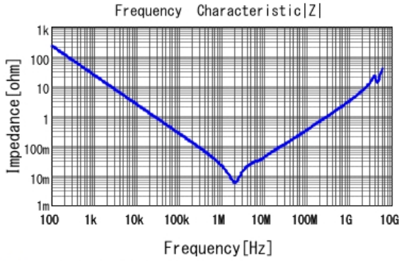
■ GRM31MR61C106KA12 |Z| DCOV, 25degC
