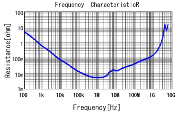
■ GRM31MR61C106KA12 R DCOV, 25degC
