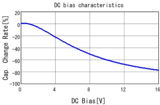
■ GRM31MR61C106KA12 C-DC bias capchange, 25.0degC, AC1.
