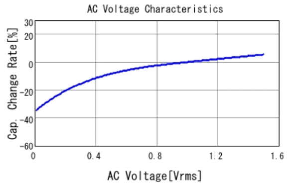
■ GRM31MR61C106KA12 C-AC Voltage capchange, DCOV, 25.0d
