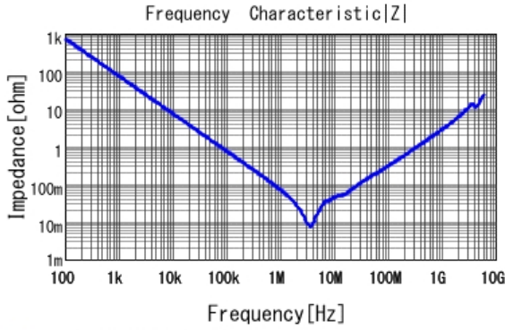
■ GRM31MR11E225KA93 |Z| DCOV, 20degC
