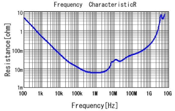
■ GRM31MR11E225KA93 R DCOV, 20degC
