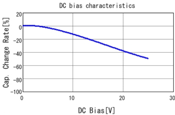
■ GRM31MR11E225KA93 C-DC bias capchange, 20.0degC, AC1.
