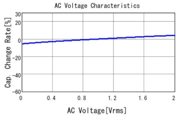
■ GRM31MR11E225KA93 C-AC Voltage capchange, DCOV, 20.0d
