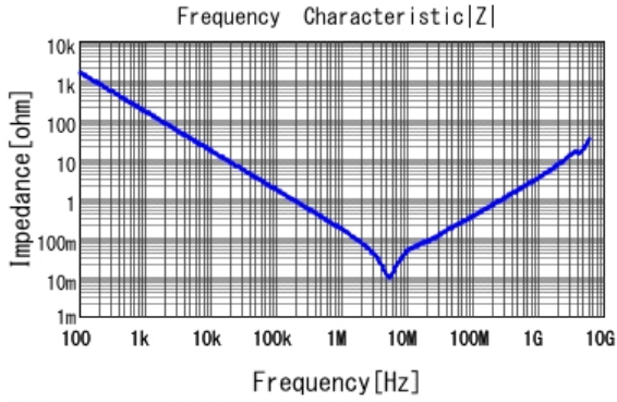
■ GRM31MB31H105KA87 |Z| DCOV, 20degC
