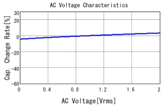
■ GRM31MB31H105KA87 C-AC Voltage capchange, DCOV, 20.0d
