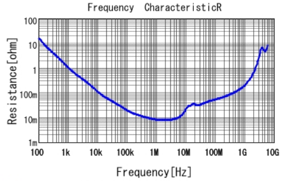
■ GRM31MB31H105KA87 R DCOV, 20degC
