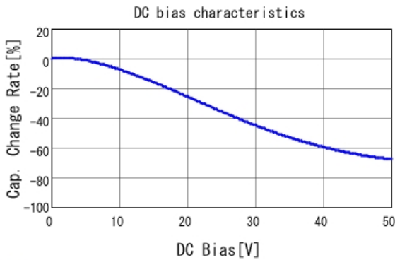
■ GRM31MB31H105KA87 C-DC bias capchange, 20.0degC, AC1.
