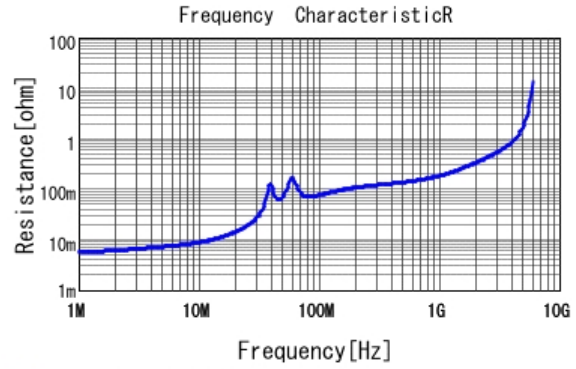
■ GRM31M7U1H823JA01 R DCOV, 25degC
