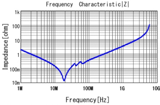
■ GRM31M7U1H823JA01 |Z| DCOV, 25degC
