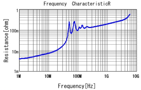
■ GRM31M5C2A473JA01 R DC0V, 25degC
