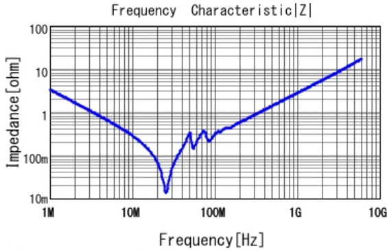
■ GRM31M5C2A473JA01 |Z| DC0V, 25degC
