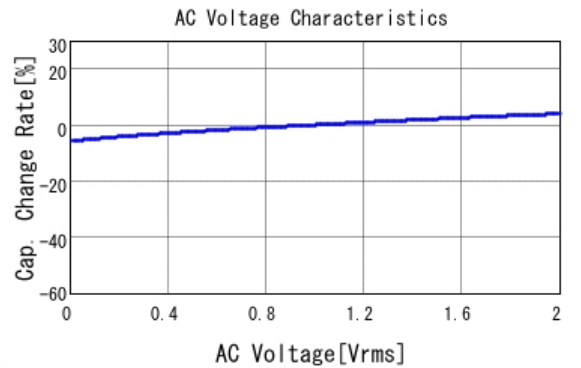
■ GRM31CZ72A475KE11 C-AC Voltage capchange, DCOV, 25.0d
