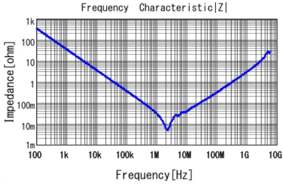
■ GRM31CZ72A475KE11 |Z| DCOV, 25degC
