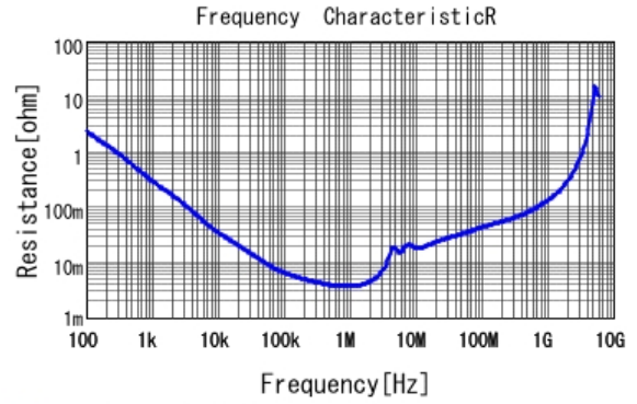
■ GRM31CZ72A475KE11 R DCOV, 25degC
