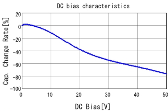
■ GRM31CR71H475MA12 C-DC bias capchange, 25.0degC, AC1.
