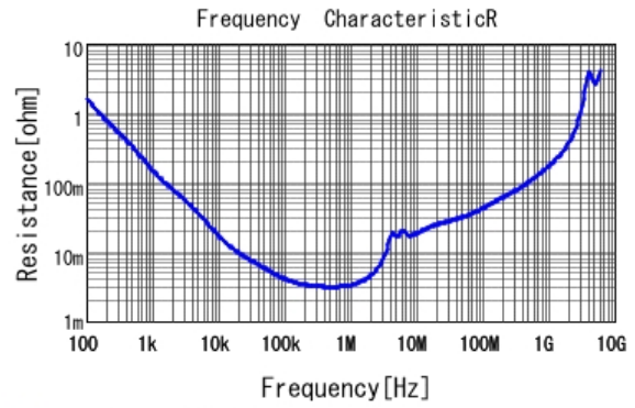
■ GRM31CR71H475MA12 R DCOV, 25degC
