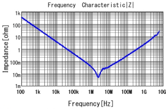
■ GRM31CR71H475MA12 |Z| DCOV, 25degC
