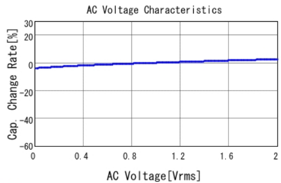
■ GRM31CR71H475MA12 C-AC Voltage capchange, DCOV, 25.0d
