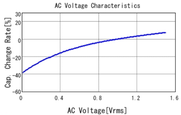
■ GRM31CR71E106MA12 C-AC Voltage capchange, DCOV, 25.0d
