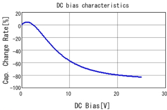
■ GRM31CR71E106MA12 C-DC bias capchange, 25.0degC, AC1.
