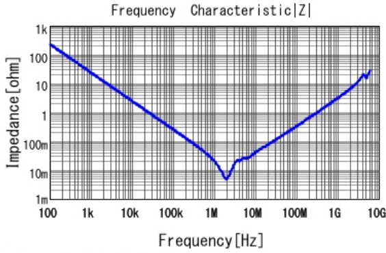
■ GRM31CR71E106MA12 |Z| DCOV, 25degC
