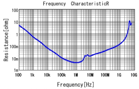
■ GRM31CR71E106MA12 R DCOV, 25degC
