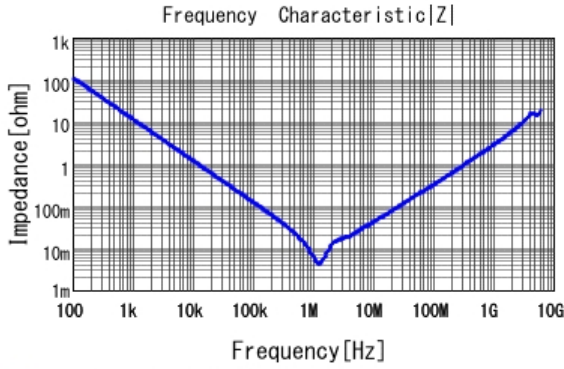
■ GRM31CR70J226ME19 |Z| DCOV, 25degC
