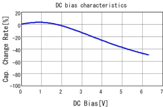
■ GRM31CR70J226ME19 C-DC bias capchange, 25.0degC, AC0.
