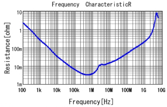
■ GRM31CR70J226ME19 R DCOV, 25degC
