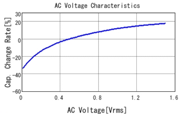
■ GRM31CR70J226ME19 C-AC Voltage capchange, DCOV, 25.0d
