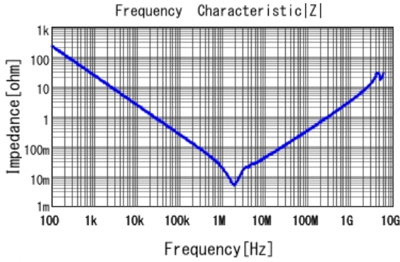
■ GRM31CR61H106MA12 |Z| DCOV, 25degC
