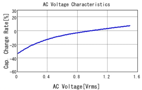
■ GRM31CR61H106MA12 C-AC Voltage capchange, DCOV, 25.0d
