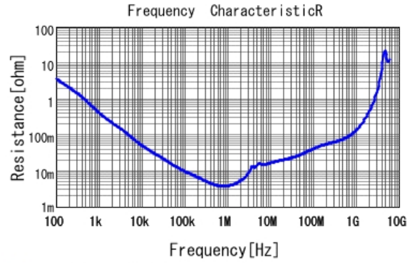
■ GRM31CR61H106MA12 R DCOV, 25degC
