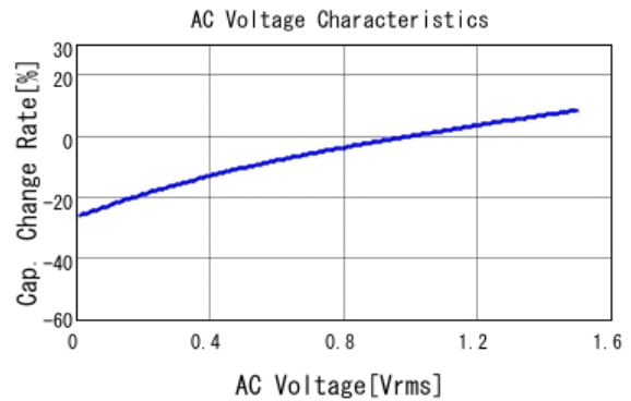
■ GRM31CR61E106MA12 C-AC Voltage capchange, DCOV, 25.0d
