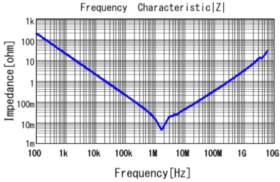
■ GRM31CR61E106MA12 |Z| DCOV, 25degC
