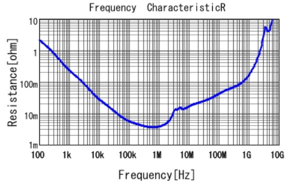
■ GRM31CR61E106MA12 R DCOV, 25degC
