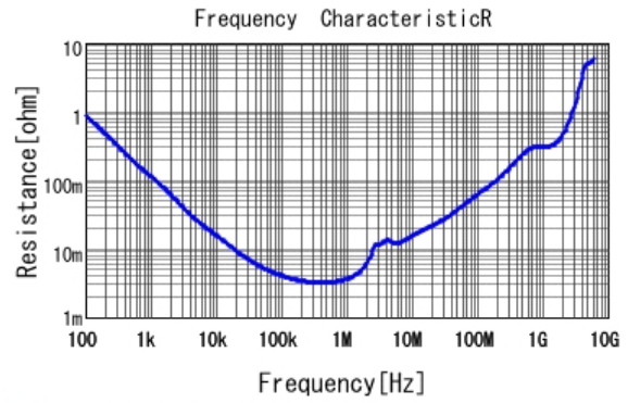
■ GRM31CR61C106KC31 R DCOV, 25degC
