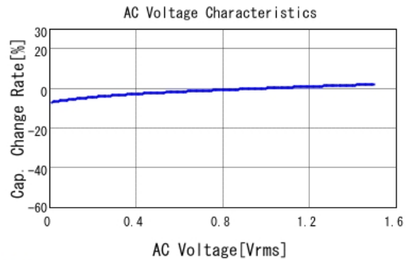
■ GRM31CR61C106KC31 C-AC Voltage capchange, DCOV, 25.0d
