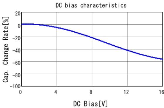
■ GRM31CR61C106KC31 C-DC bias capchange, 25.0degC, AC1.
