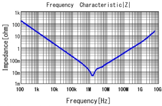
■ GRM31CR61C106KC31 |Z| DCOV, 25degC
