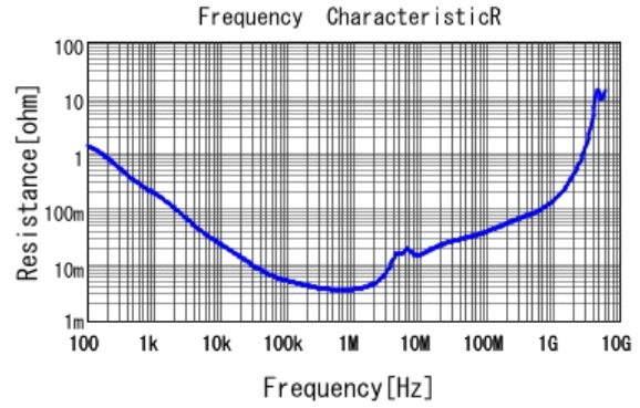
■ GRM31CR60J475KA01 R DCOV, 25degC
