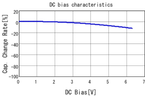
■ GRM31CR60J475KA01 C-DC bias capchange, 25.0degC, AC1.
