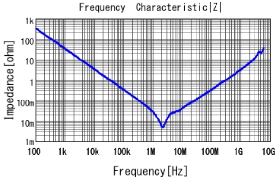
■ GRM31CR60J475KA01 |Z| DCOV, 25degC
