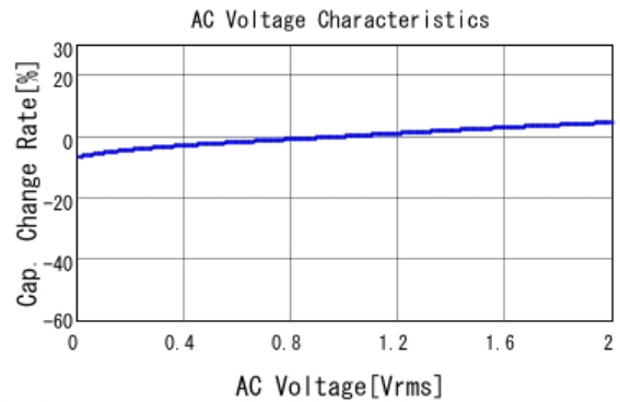
■ GRM31CR60J475KA01 C-AC Voltage capchange, DCOV, 25.0d
