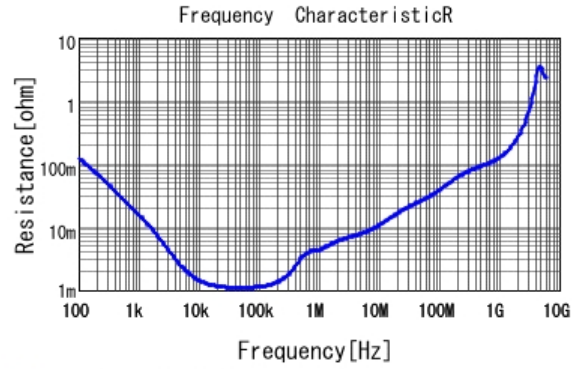
■ GRM31CR60G227ME11 R DCOV, 25degC
