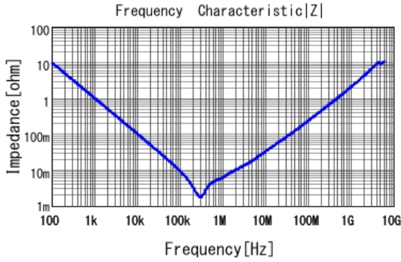
■ GRM31CR60G227ME11 |Z| DCOV, 25degC
