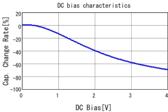
■ GRM31CR60G227ME11 C-DC bias capchange, 25.0degC, AC0.
