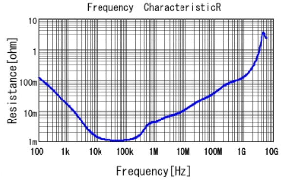
■ GRM31CR60E227ME11 R DCOV, 25degC
