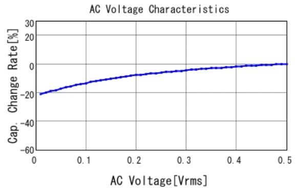
■ GRM31CR60E227ME11 C-AC Voltage capchange, DCOV, 25.0d
