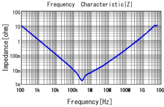
■ GRM31CR60E227ME11 |Z| DCOV, 25degC
