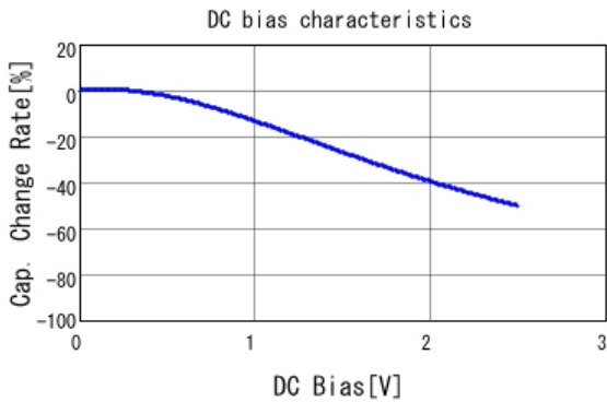
■ GRM31CR60E227ME11 C-DC bias capchange, 25.0degC, AC0.
