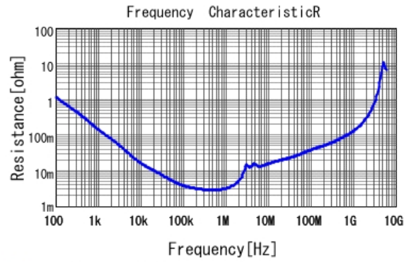
■ GRM31CD71H106KE11 R DCOV, 25degC
