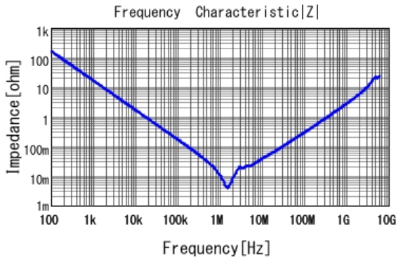
■ GRM31CD71H106KE11 |Z| DCOV, 25degC
