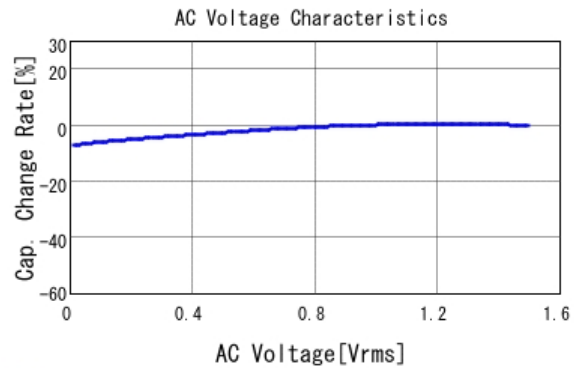
■ GRM31CD71H106KE11 C-AC Voltage capchange, DCOV, 25.0d
