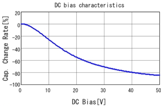
■ GRM31CD71H106KE11 C-DC bias capchange, 25.0degC, AC1V
